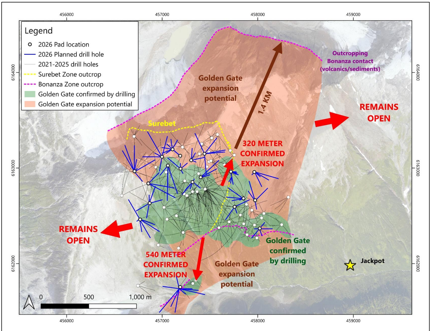
Figure 1a. Golden Gate Expansion Map
