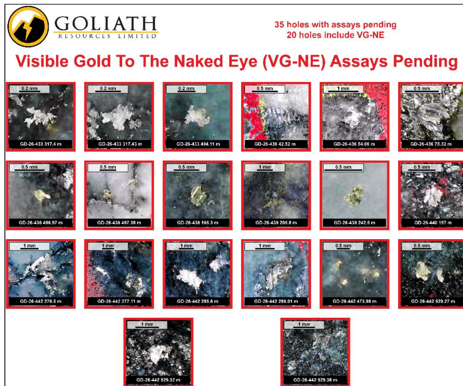
Figure 4c. Visible Gold to the Naked Eye (VG-NE) cont'
