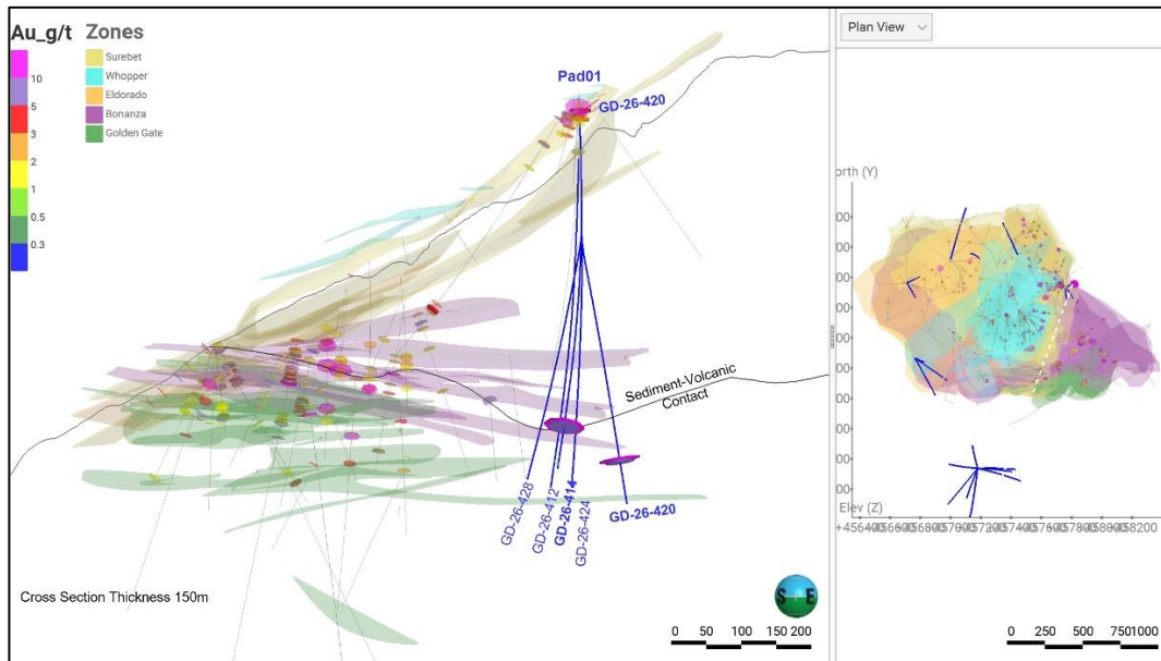
Figure 1b. Cross Section
