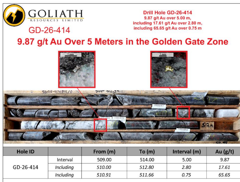
Figure 2a. Highlights of Hole GD-26-414 – Golden Gate Zone
