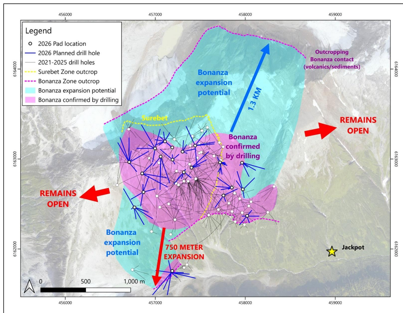
5. Plan View showing the expanded Bonanza Zone
