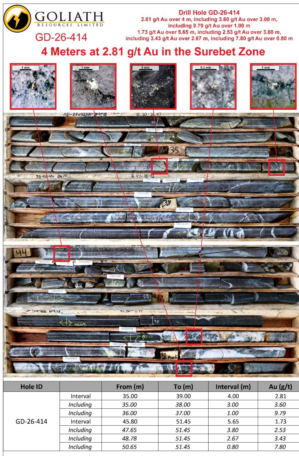
Figure 2b. Highlights of Hole GD-26-414 – Surebet Zone
